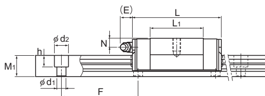
Model GSR25V-R
