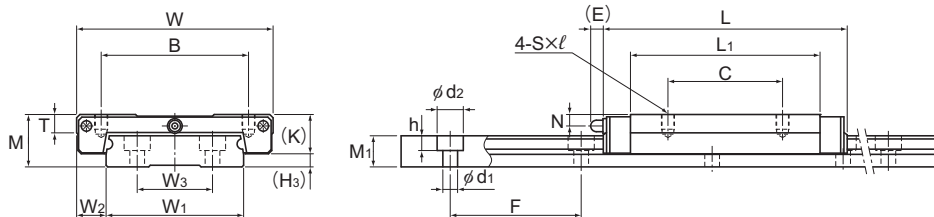
Models RSR15M1WV/M1WV
