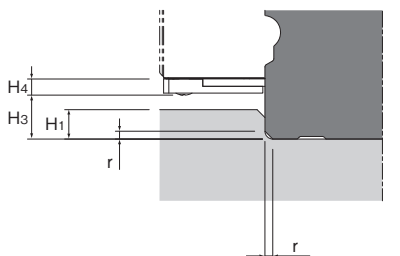
Side view of the LM block after the protector and side scraper are mounted
