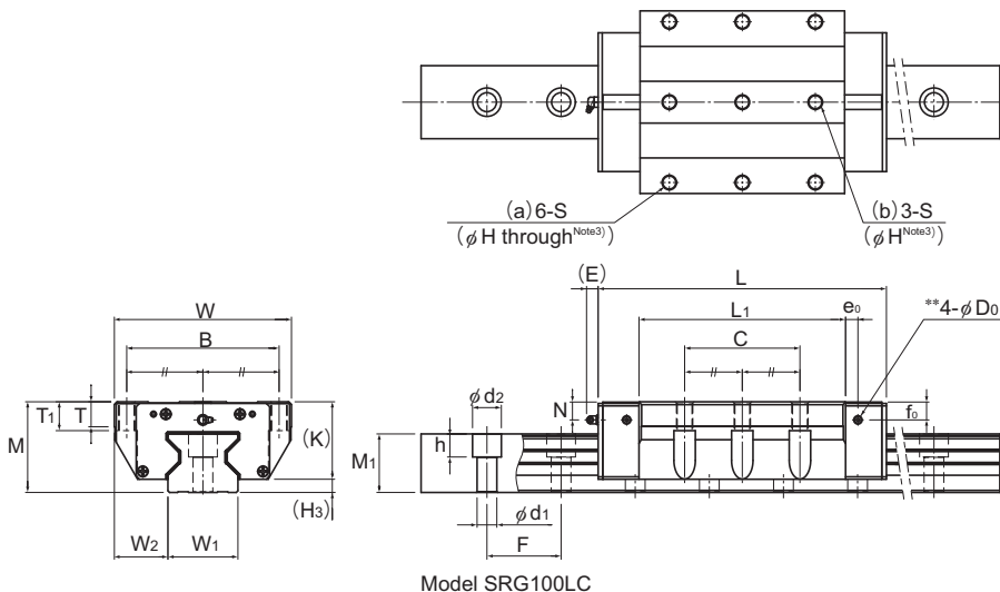
Model SRG100LC
