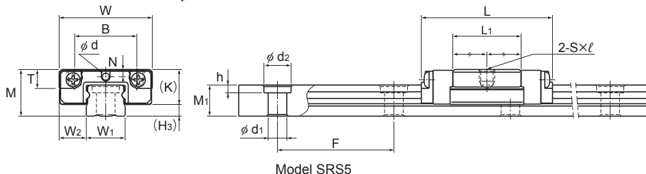
Model SRS5
