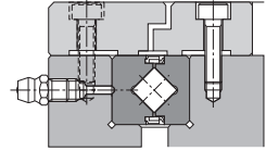
Example 2 of assembling model RB
