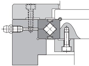
Example 1 of assembling model RB
